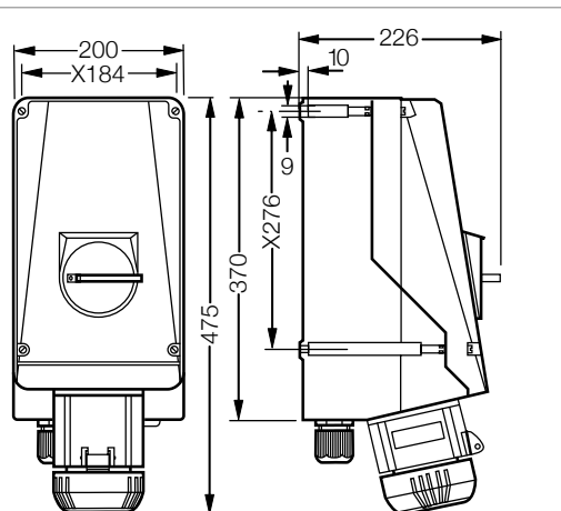
Wall socket 4/5-pole
